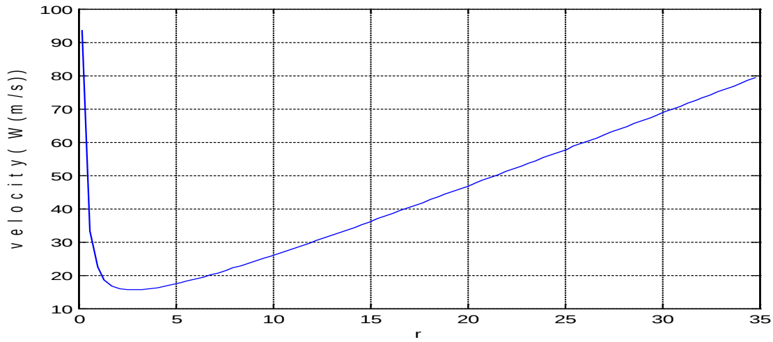
Figure 2.3. Velocity variation along the span
