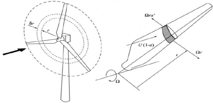
Figure 2.1. A blade element sweep out an angular ring [1]
