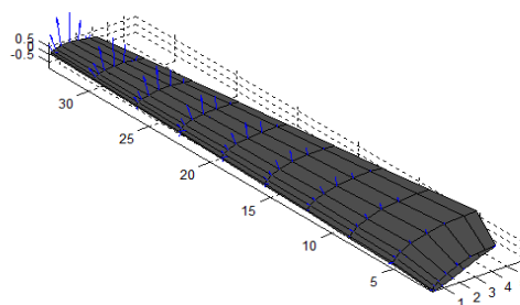
Figure 4.4. Local forces
