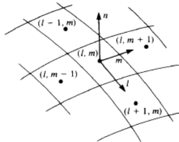
Figure 3.6. Nomenclature used for the differentiation of the velocity potential for local tangential velocity calculations [4]
