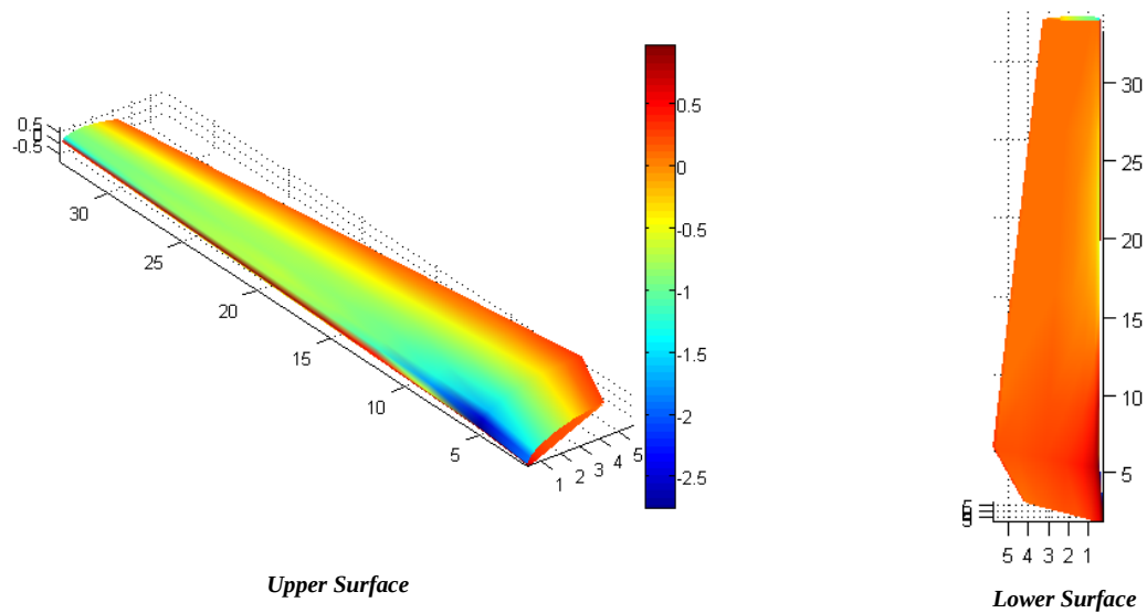
Figure 4.2. Pressure Coefficients
