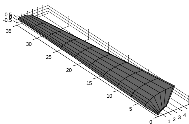
Figure 4.1. Blade Geometry (Practical Chord)
