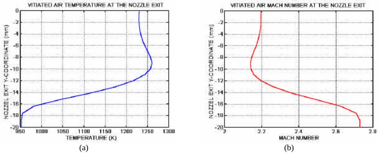
Fig. 6 Values of the vitiated air temperature and Mach number at the nozzle exit. (nozzle centerline: Y = 0 mm)
