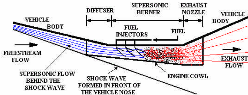
Fig. 2 Schematic drawing of a scramjet combustor (Curran, 1996).
