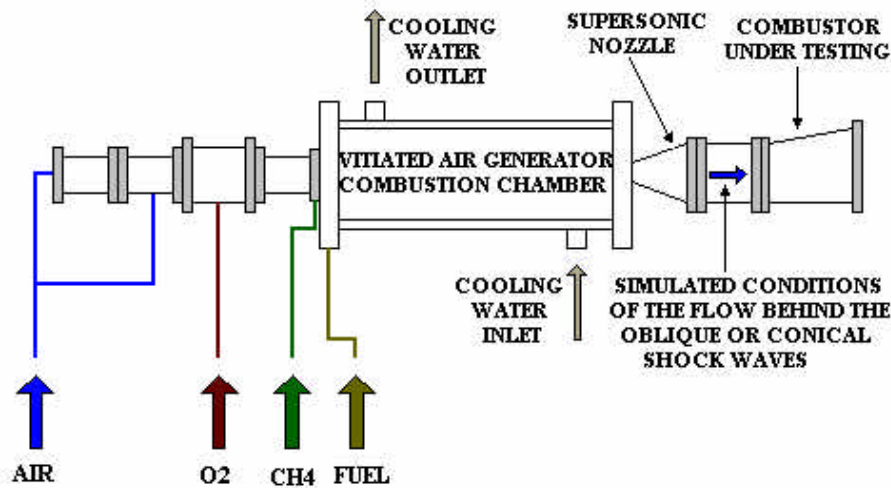
Fig. 1 Schematic drawing of supersonic combustion research facility.
