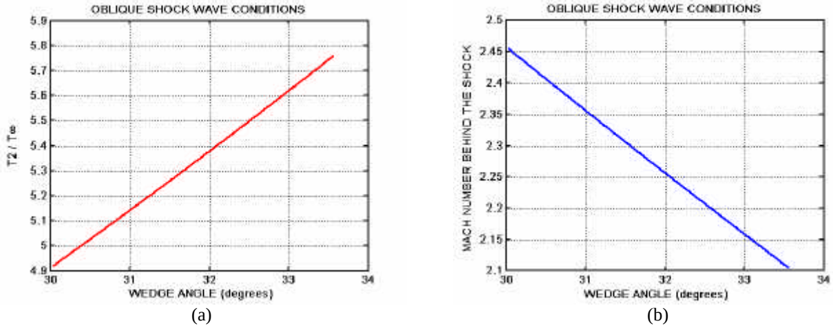
Fig. 4 Flow conditions behind an oblique shock wave for the free stream Mach number 7.
