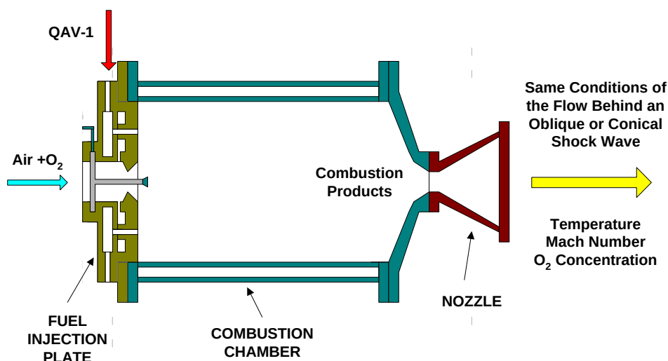
Fig. 3 Schematic drawing of the vitiated air generator with the nozzle.
