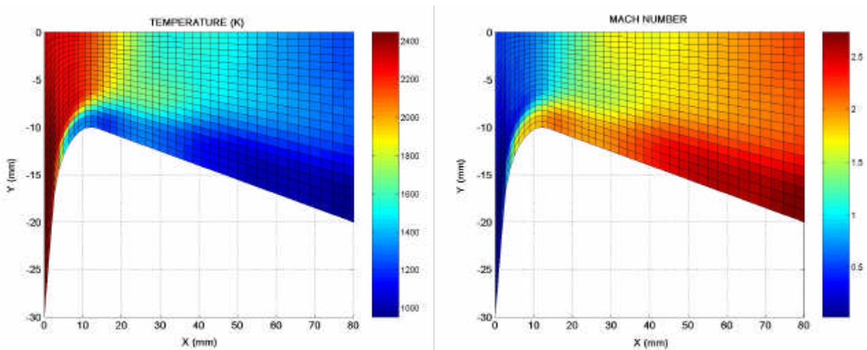
Fig. 5 Temperature and Mach number distribution inside the nozzle. (nozzle centerline: Y = 0 mm)
