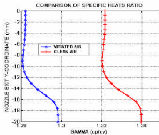
Fig. 7 Comparison between the specific heats ratio of the vitiated and the clean air at the nozzle exit.
