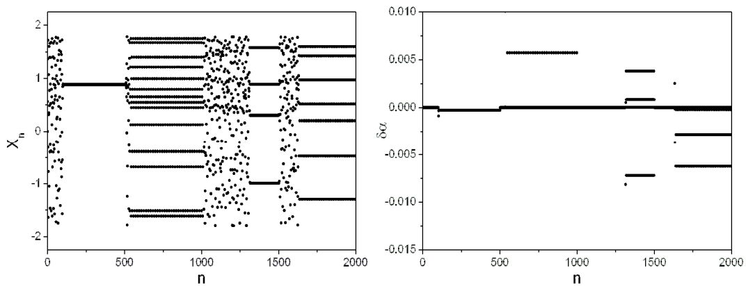
Figure 3. Hénon map stabilization using single-parameter \delta\alpha : (a) Displacement; (b) Control parameters perturbations.
