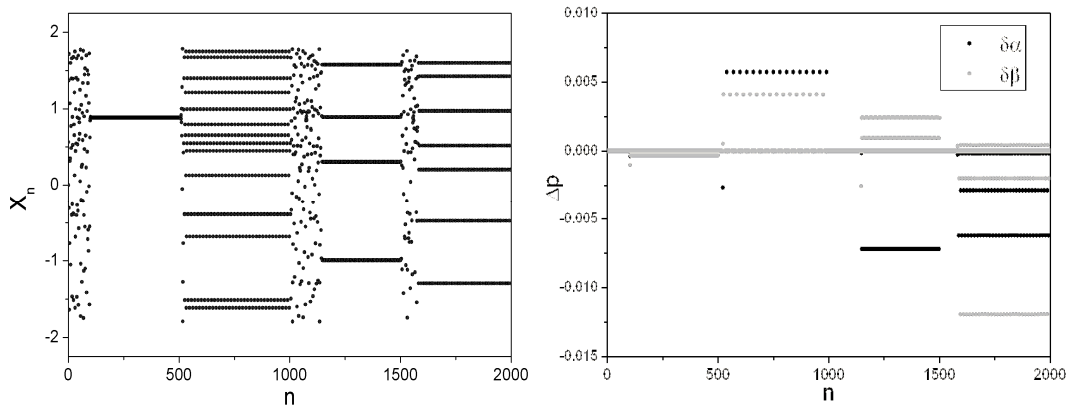
Figure 2. Hénon map stabilization using uncoupled multiparameter approach: (a) Displacement; (b) Control parameters perturbations.
