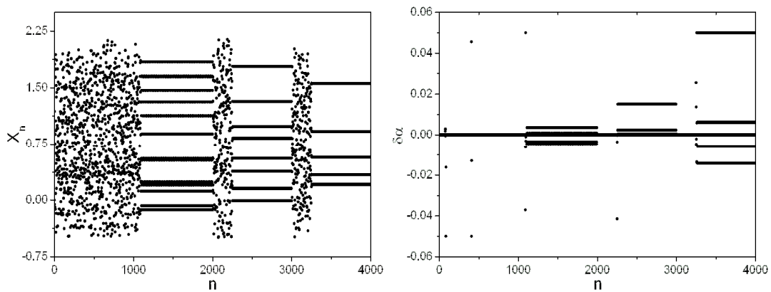
Figure 7. Ikeda map stabilization using single-parameter \delta\alpha . (a) Displacement; (b) Control parameters perturbations.
