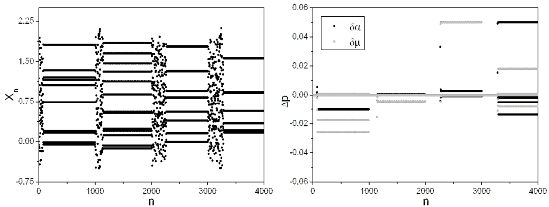
Figure 6. Ikeda map stabilization using uncoupled multiparameter approach: (a) Displacement; (b) Control parameters perturbations.
