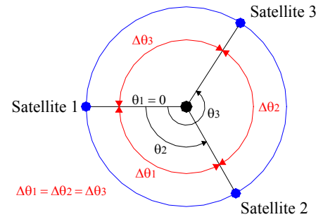
Fig. 2 – Nominal position of the satellites.
