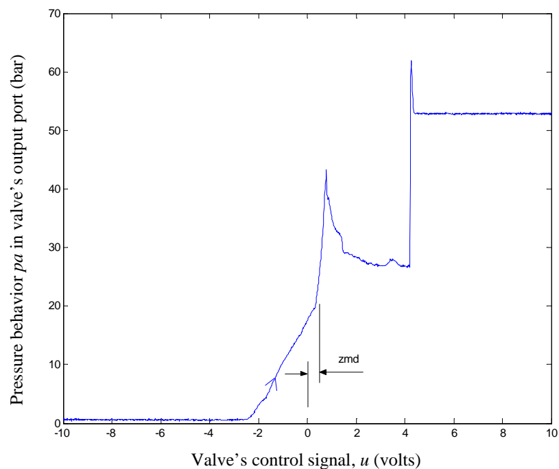
Figure 7. Pressure behavior p_a in valve's output port and the evidence of the right dead zone value.
