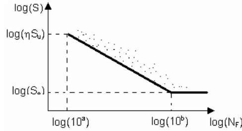
Figure 5: Typical S-N F curve.
