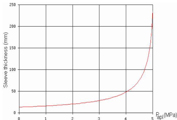
Figure 2: Influence of the internal pressure P_{\text{apl}} in the sleeve thickness to assure a maximum hoop stress \sigma_{\text{Max}} = 146.3 MPa in the pipe. P_i = 5 MPa.
