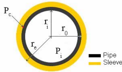
Figure 1: Pipe and sleeve with internal pressure
