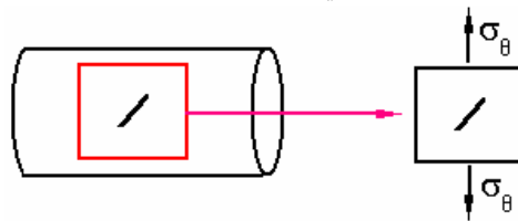
Figure 6: Approximate problem.
