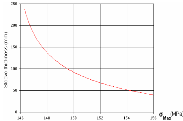
Figure 3: Influence of \sigma_{Max} in the limit sleeve thickness for P_{apl} = 5 MPa and P_0 = 7.2 MPa.
