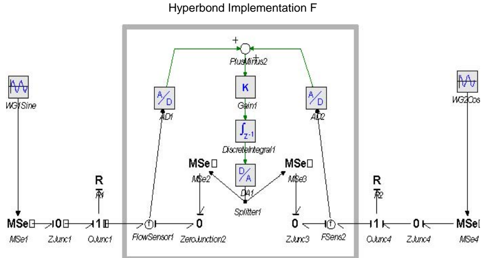
Figure 6. Hyper-bond implementation
