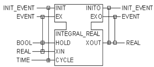
Fig.10 – Function Bloc –FB
