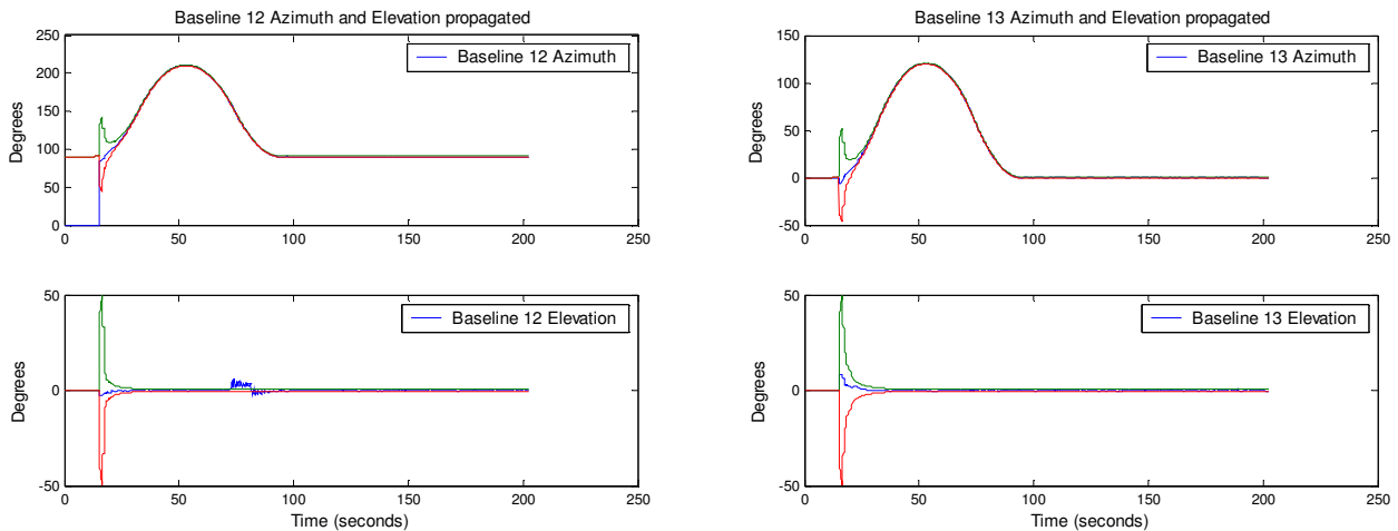
Figure 5. 3-axis filtered and propagated attitude, 1 sigma. (Attitude matrix transformed for azimuth and elevation).
