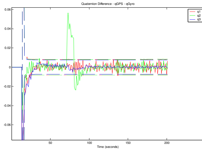
Figure 7. Difference between GPS estimated quaternion and Gyro propagated quaternion, 1 sigma.
