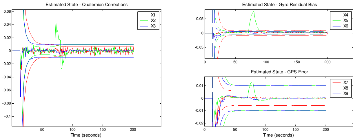
Figure 6. State Estimated, 1 sigma.
