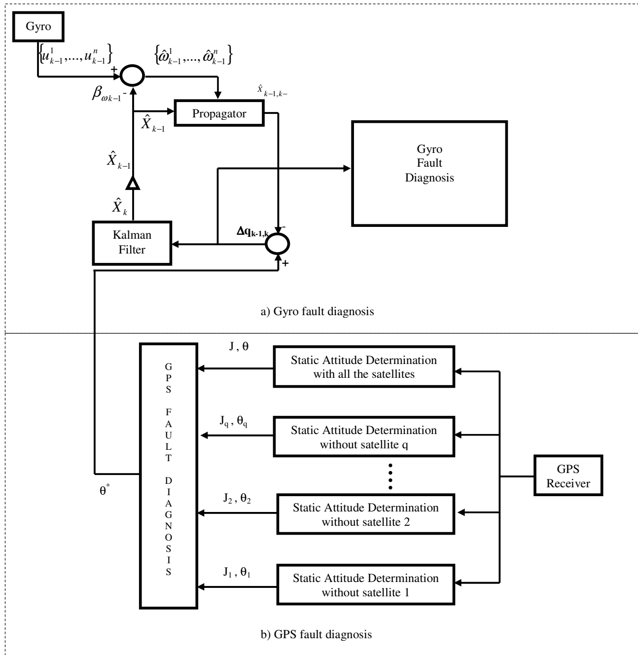
Figure 2. Fault diagnosis algorithm schema.
