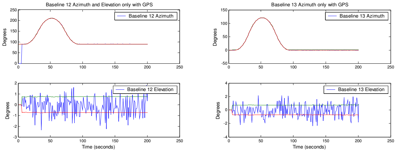
Figure 4. 3-axis attitude estimated using only GPS, 1 sigma. (Attitude matrix transformed for azimuth and elevation).
